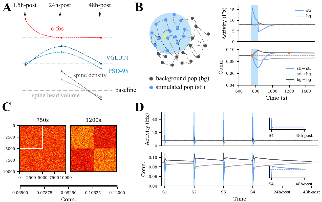
Figure 6. The HSP model. (A) The interpolated time course of the expression of c-Fos , VGLUT1, PSD-95, and spine morphology compared with sham (baseline). (B) Temporal evolution of neural activity and network connectivity in response to optogenetic stimulation. Light blue shaded areas indicate the stimulation period. Blue and dark gray curves in the upper panel represent the firing rate of stimulated and nonstimulated neurons. Blue, dark gray, and light gray curves in the lower panel represent the synaptic connectivity within or between populations. The blue and light gray curves finally coincided due to identical population sizes. (C) The connection matrix of all excitatory neurons at two time points before and after stimulation, labeled by orange dots in panel B. Columns are the presynaptic neurons, and rows are the postsynaptic neurons. Color indicates the average connectivity. The white square labels the intragroup connectivity of the stimulated neurons. (D) Repetitive optogenetic stimulation boosted the connectivity among the stimulated neurons. Small insets display the dynamics within 48 h after the last stimulation session.
