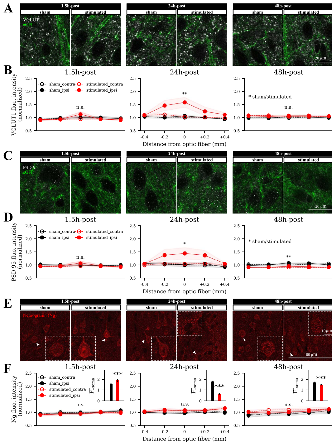
Figure 2. Optogenetic stimulation altered the expression of VGLUT1 and PSD-95 and the cellular translocation of neurogranin. (A, C, E) Representative images of VGLUT1, PSD-95, and neurogranin staining on the ipsilateral hemisphere of sections within 0.1 mm AP to the optic fiber from both sham and stimulated mice. The insets in panel (E) display the example neurons. (B) Normalized VGLUT1 fluorescent intensity at different times and different distances to the fiber optic. The main effect of optogenetic stimulation (sham/stimulated) was significant at 24 h. (D) The PSD-95 fluorescent intensity at different times and distances. At 24 h and 48 h, the main effect of stimulation was significant. (F) The overall fluorescent intensity of neurogranin was not changed by stimulation (LMM), while the relative intensity of neural soma ( FI_{soma} ) from the stimulated mice was slightly increased at 1.5h, greatly dropped below 1 at 24h, and recovered to a level lower than sham at 48 h ( P < 0.001 , P < 0.001 , P < 0.001 , respectively, Mann-Whitney U test).
