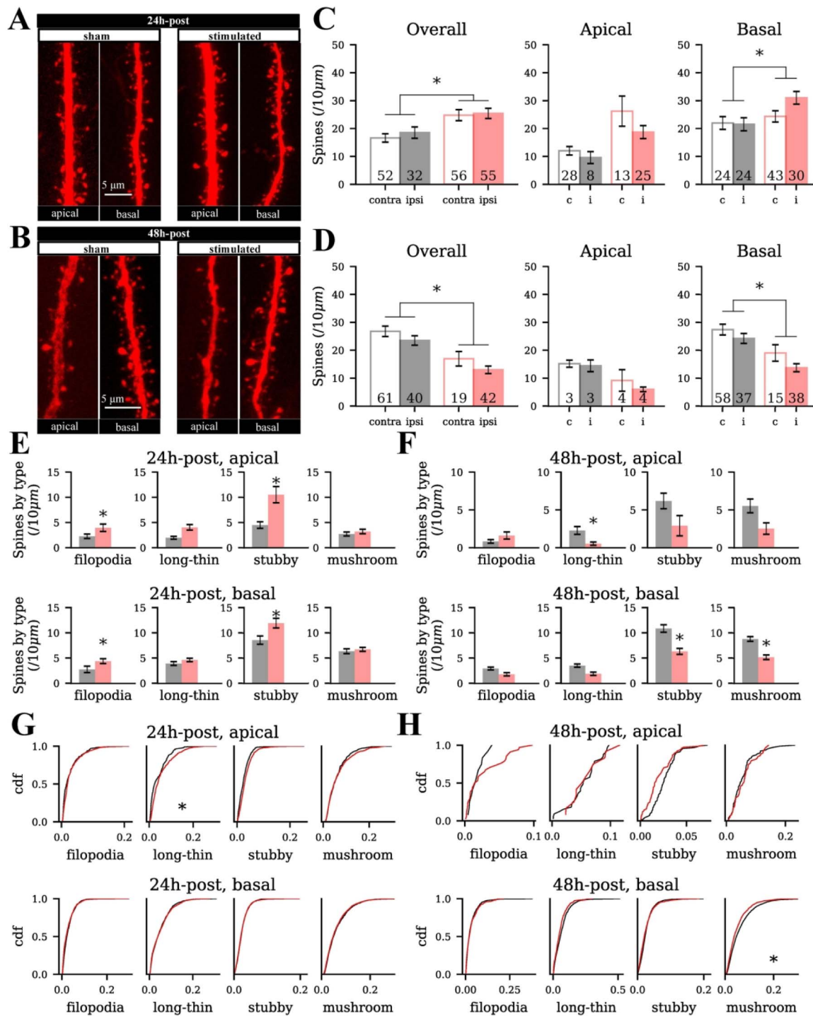
Figure 4. Spine density and head volume showed the opposite changes at 24 h and 48 h post-stimulation. (A–B) Representative example of filled dendritic segments. (C–D) Spine density at 24 h (84 dendritic segments from sham and 111 segments from stimulated mice) and 48 h (101 segments from sham and 61 segments from stimulated mice). (E–F) Spine density of each class. (G–H) Cumulative distribution of spine head volume. LMM was used for statistical analysis.
