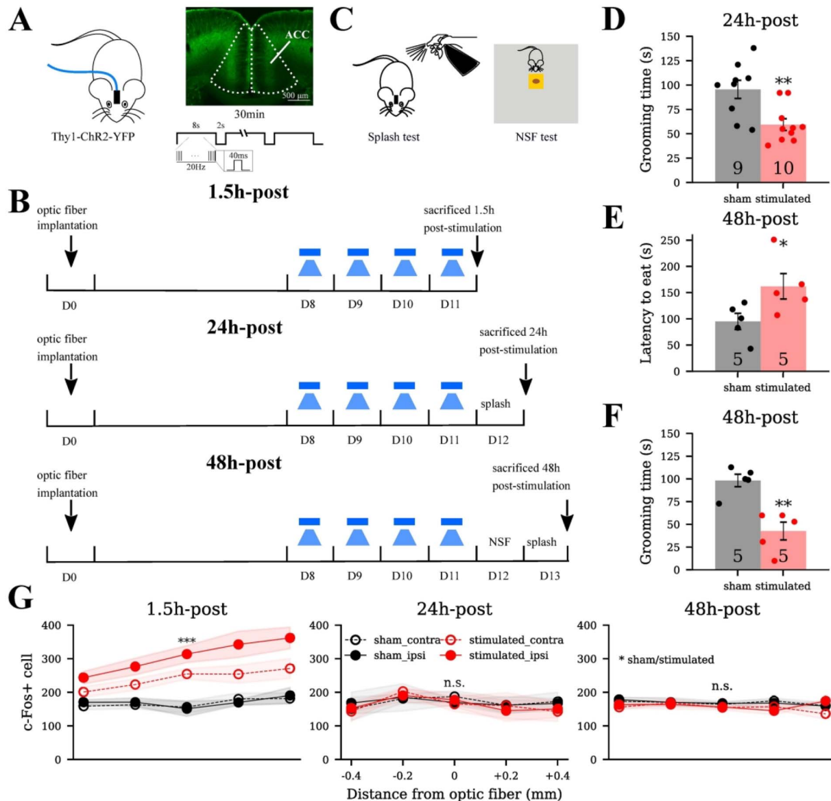
Figure 1. Consecutive optogenetic stimulation triggered hyperactivity in ACC and depressive-like behavior in mice. (A–C) Experimental design of the current study. (D–F) Mice used for immunohistochemical staining experiments showed depressive-like behavior at 24 h and 48 h post-stimulation. (D) Splash test results of mice sacrificed at 24 h post-stimulation ( P = 0.003 , Mann–Whitney U test; N = 9 for sham, N = 10 for stimulated mice). (E–F) Results of NSF and splash tests for mice sacrificed at 48 h ( P = 0.01 and P = 0.005 , Mann–Whitney U test; N = 5 for sham, N = 5 for stimulated mice). (G) c-Fos expression was elevated by the optogenetic stimulation at 1.5 h ( P < 0.001 ) and specifically on the ipsilateral side ( P < 0.01 ), decayed to baseline at 24 h and 48 h post-stimulation. The x ticks label the mean distance of stained sections (–, anterior; +, posterior) from the optical fiber. The y axis labels the c-Fos+ cell number within the masks of stained sections. GLMM was used for the statistical analysis. P < 0.05 , P < 0.01 , and P < 0.001 means 95% CI, 99% CI, and 99.9% CI does not cross zero, respectively.
