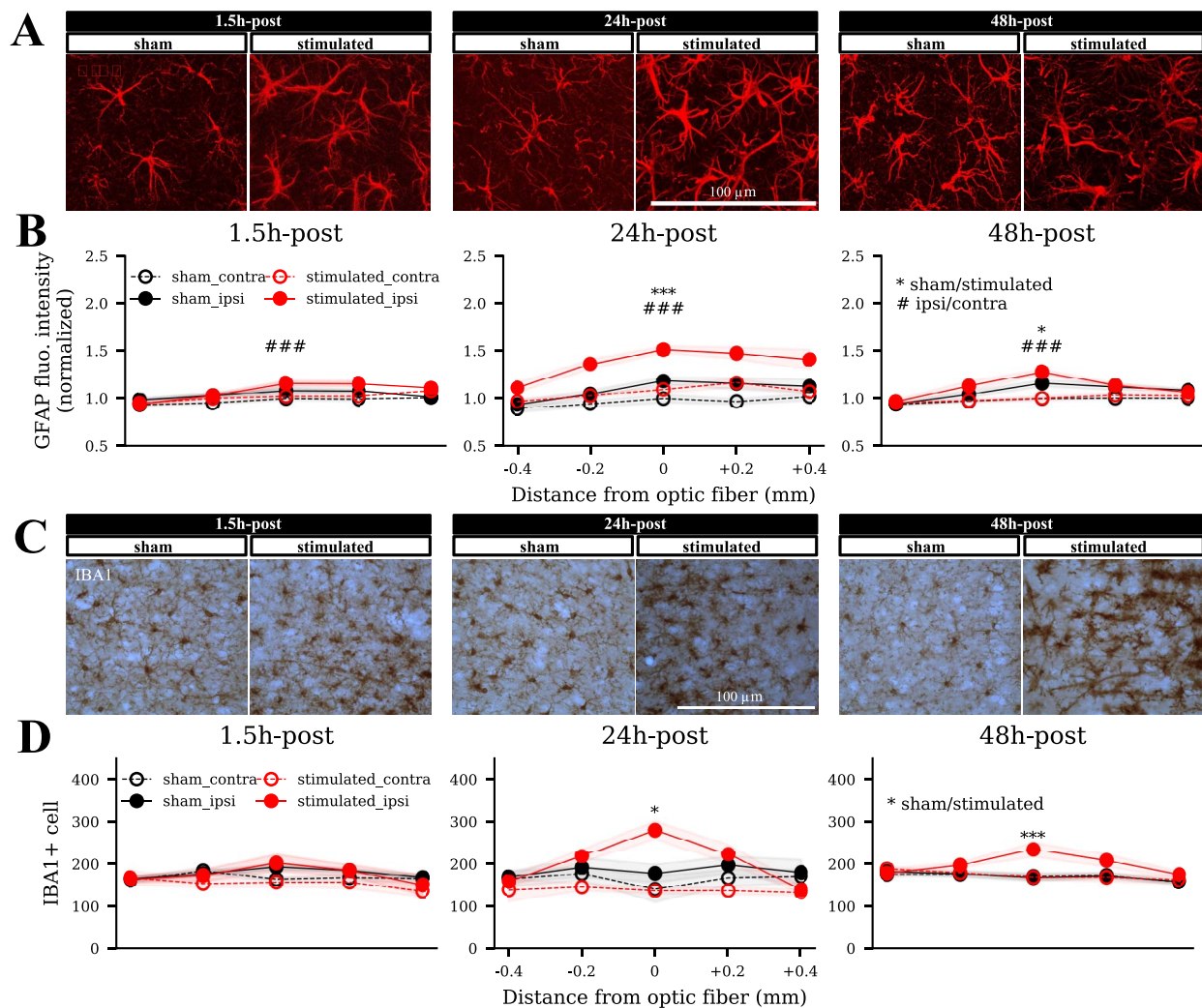
Figure 5. Expression of GFAP and IBA1 were upregulated by optogenetic stimulation at 24 h and 48h post-stimulation. (A) and (C) Representative images of GFAP and IBA1 staining on the ipsilateral hemisphere of sections within 0.1 mm AP to the optic fiber from both sham and the stimulated mice. (B) The normalized GFAP fluorescent intensity at different time and distance. At 1.5 h, the main effect of side of implantation was significant (99.5% CI = [-0.0923, -0.0356] , LMM). At 24 h, the main effects of optogenetic stimulation and side of implantation were again significant (99.5% CI = [0.0646, 0.399] , 99.5% CI = [-0.182, -0.0628] respectively); their interaction effect was also significant (99.5% CI = [-0.264, -0.109] ). At 48 h, the main effects of stimulation, side of implantation, and their interaction effect were significant (95% CI = [0.009, 0.094] , 99.5% CI = [-0.115, -0.043] , 95% CI = [-0.079, -0.006] , respectively). (D) The IBA1+ cell counting at different time and distance to the optic fiber. At 1.5 h, only the interaction effect between stimulation and side of implantation was significant (95% CI = [-0.188, -0.00016] , GLMM). At 24 h, the main effect of optogenetic stimulation was significant (95% CI = [0.025, 0.237] ); their interaction effect was also significant (99.5% CI = [-0.533, -0.105] ). At 48 h, the main effect of optogenetic stimulation was significant (99.5% CI = [0.073, 0.193] ); their interaction effect was also significant (99.5% CI = [-0.208, -0.0369] ).
