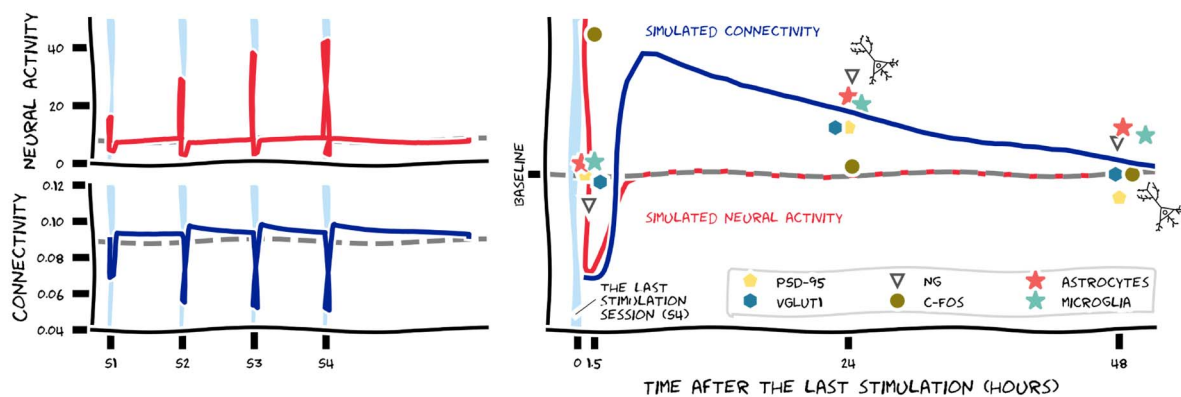
Figure 7. Joint summary of the results of mouse experiments and the computational model. Light blue shaded areas indicate four sessions of optogenetic stimulation (S1–S4, 30 min per session). Red and blue curves represent the temporal profile of neural activity and connectivity of stimulated neurons, as predicted by the model. Colored symbols in the right panel represent the expression level of c-Fos , synaptic proteins, and glial markers, respectively. Measurements were made at 1.5 h, 24 h, and 48 h post-stimulation, shown are the values from stimulated mice relative to the corresponding sham group. For Neurogranin, we show its relative expression in dendrites. The gray dashed line represents the baseline. Symbols above or below the baseline indicate that values in stimulated mice are increased or decreased as compared with sham, respectively. The illustration of a neuron with dendrites and spines depicts that spine density and spine head volume were both increased at 24 h, but decreased at 48 h post-stimulation.
